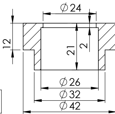
S.s. Bushing Cod.206459R
