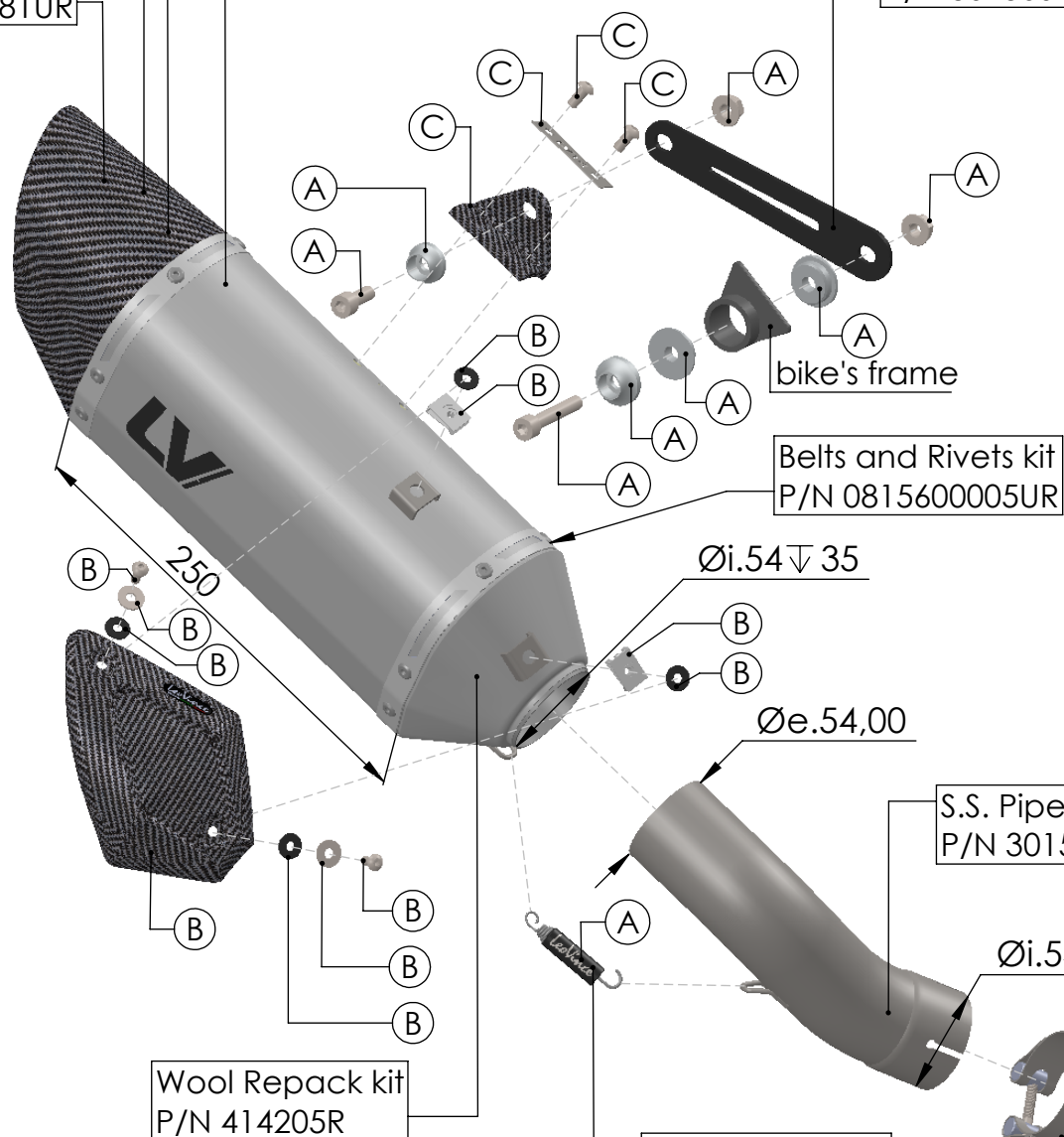
Short Spring kit P/N 303949001R
