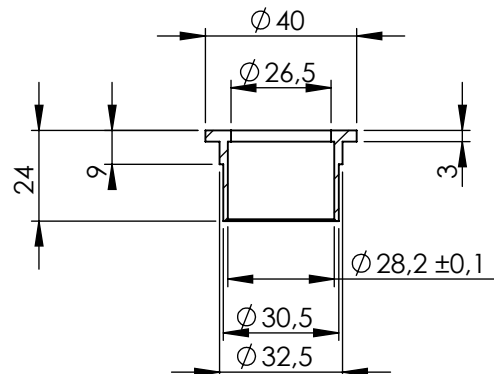
S.S. bushing P/N 206662
