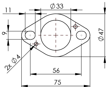
S.S. flange "45E" P/N 205267 sp. 6mm
