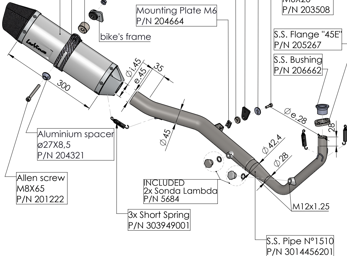
S.S. Muffler P/N 3014259481U
